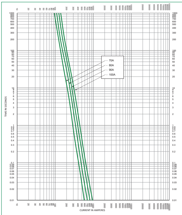
Time Current Curve JLLS (70–100 A)
