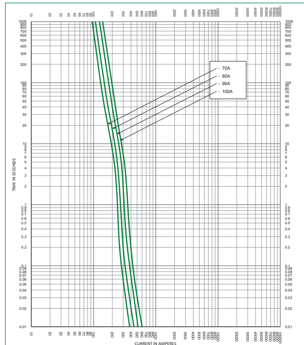
Time Current Curve JLLN (70–100 A)
