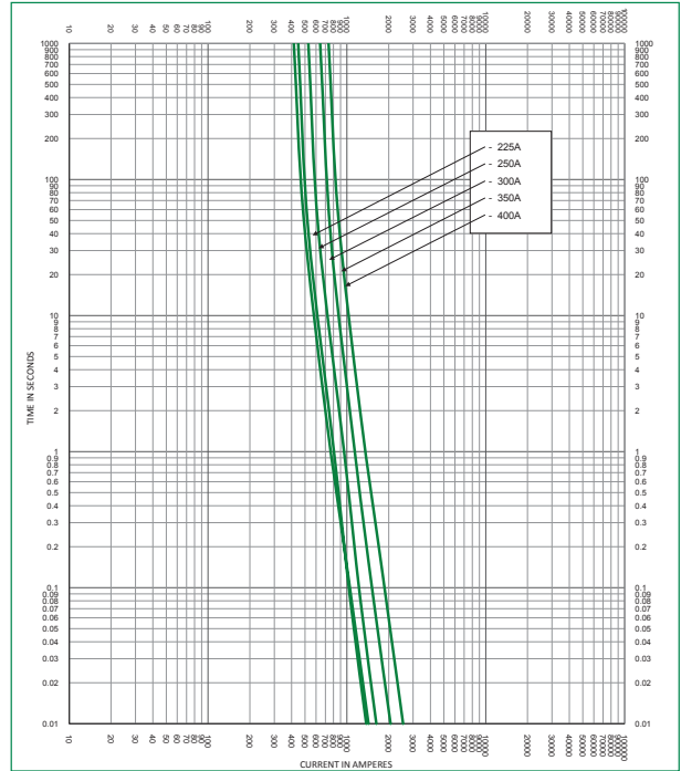
Time Current Curve JLLN (225–400 A)
