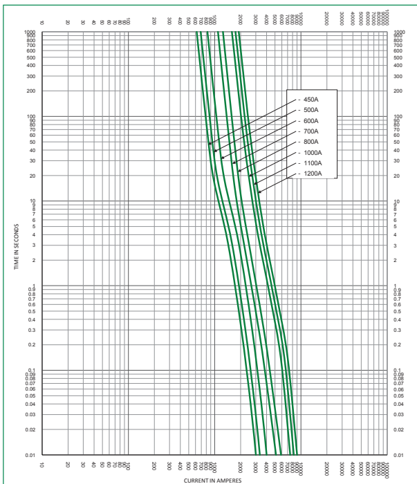
Time Current Curve JLLN (450–1200 A)
