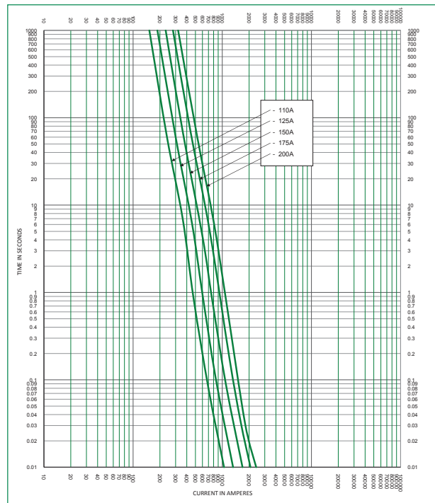
Time Current Curve JLLS (110–200 A)
