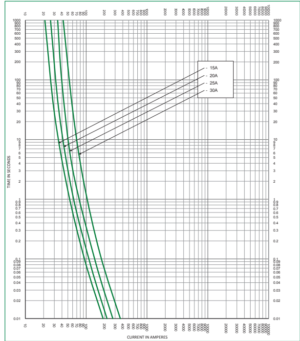
Time Current Curve JLLN (15–30 A)
