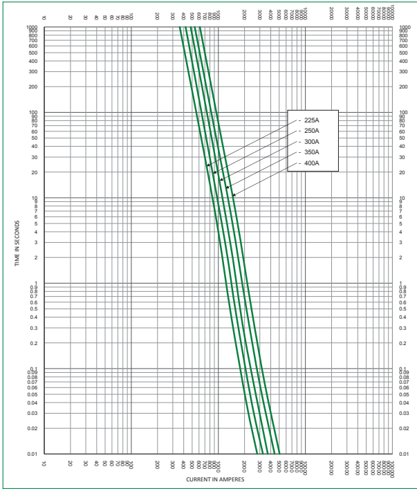
Time Current Curve JLLS (225–400A)
