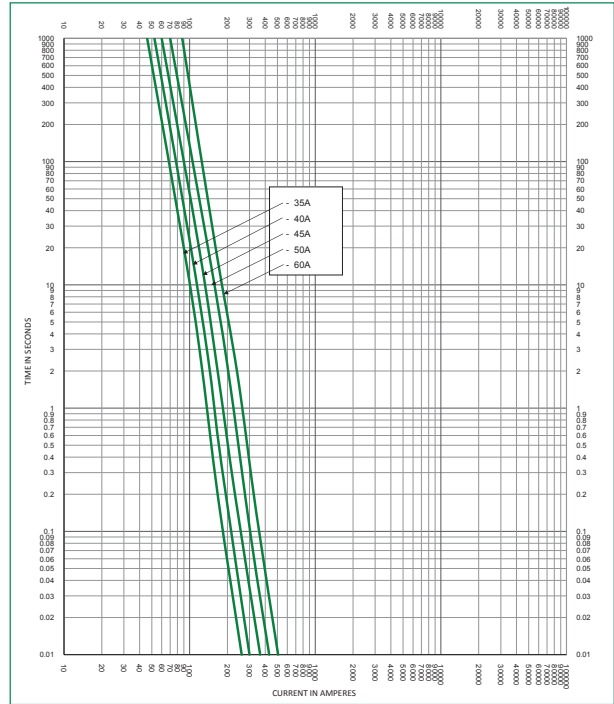
Time Current Curve JLLS (35–60 A)
