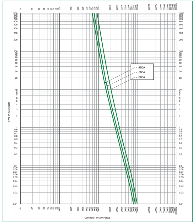
Time Current Curve JLLS (450–600A)
