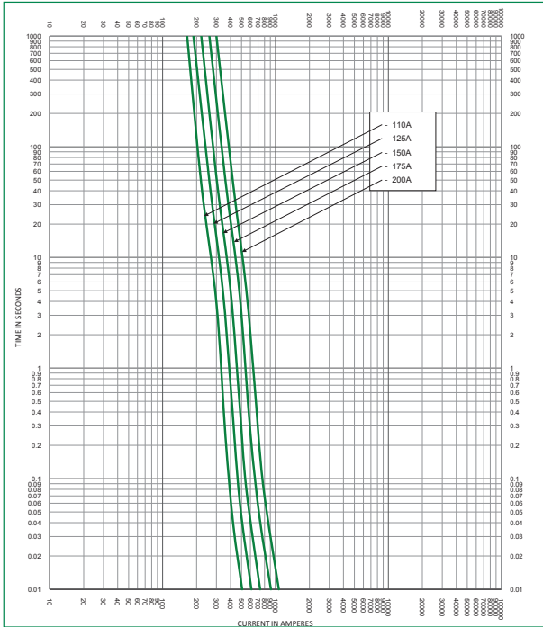
Time Current Curve JLLN (110–200 A)
