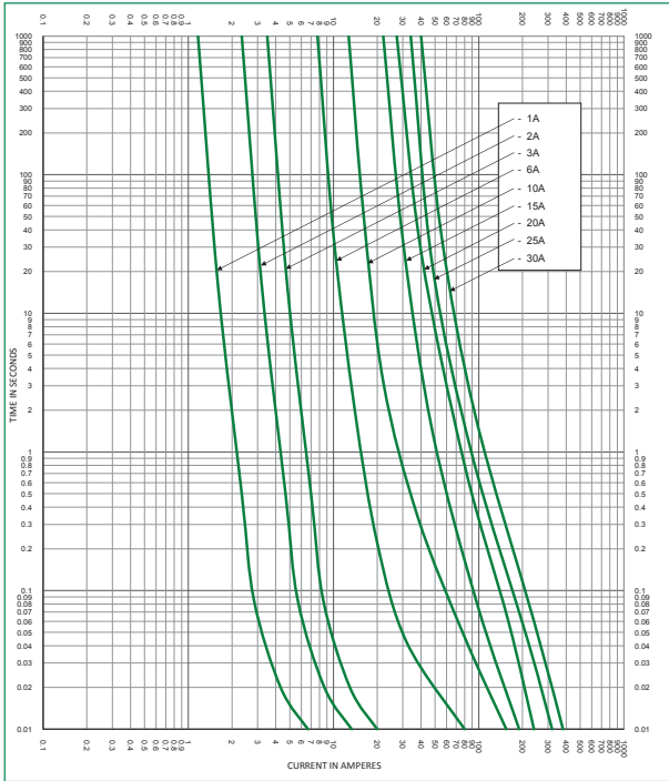
Time Current Curve JLLS (1–30 A)
