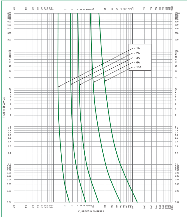
Time Current Curve JLLN (1–10 A)
