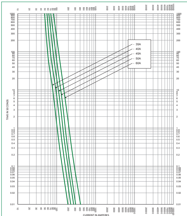
Time Current Curve JLLN (35–60 A)
