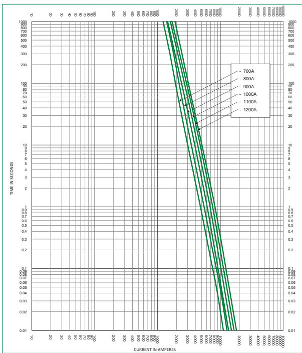
Time Current Curve JLLS (700–1200A)
